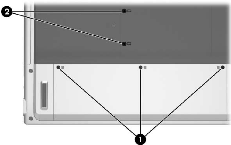
Black Phillips PM2.5x6.0 Screw Locations
