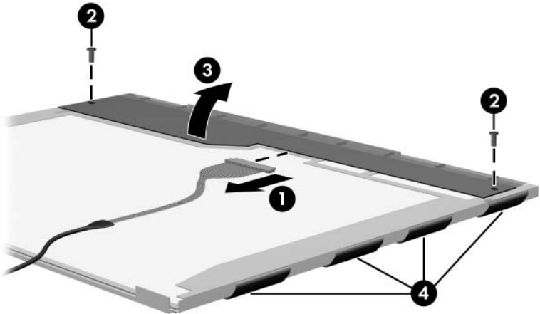
Releasing the LCD Panel
