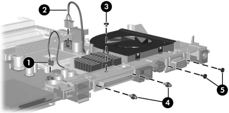
Removing the Fan Assembly Screws
