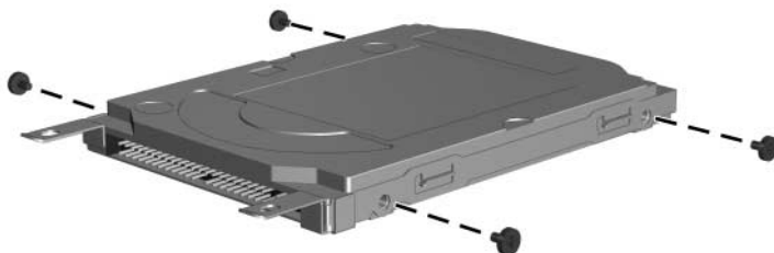
Phillips PM3.0×4.0 Screw Locations
